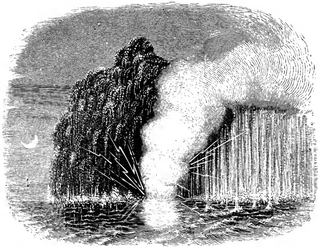
SUBMARINE VOLCANO.
